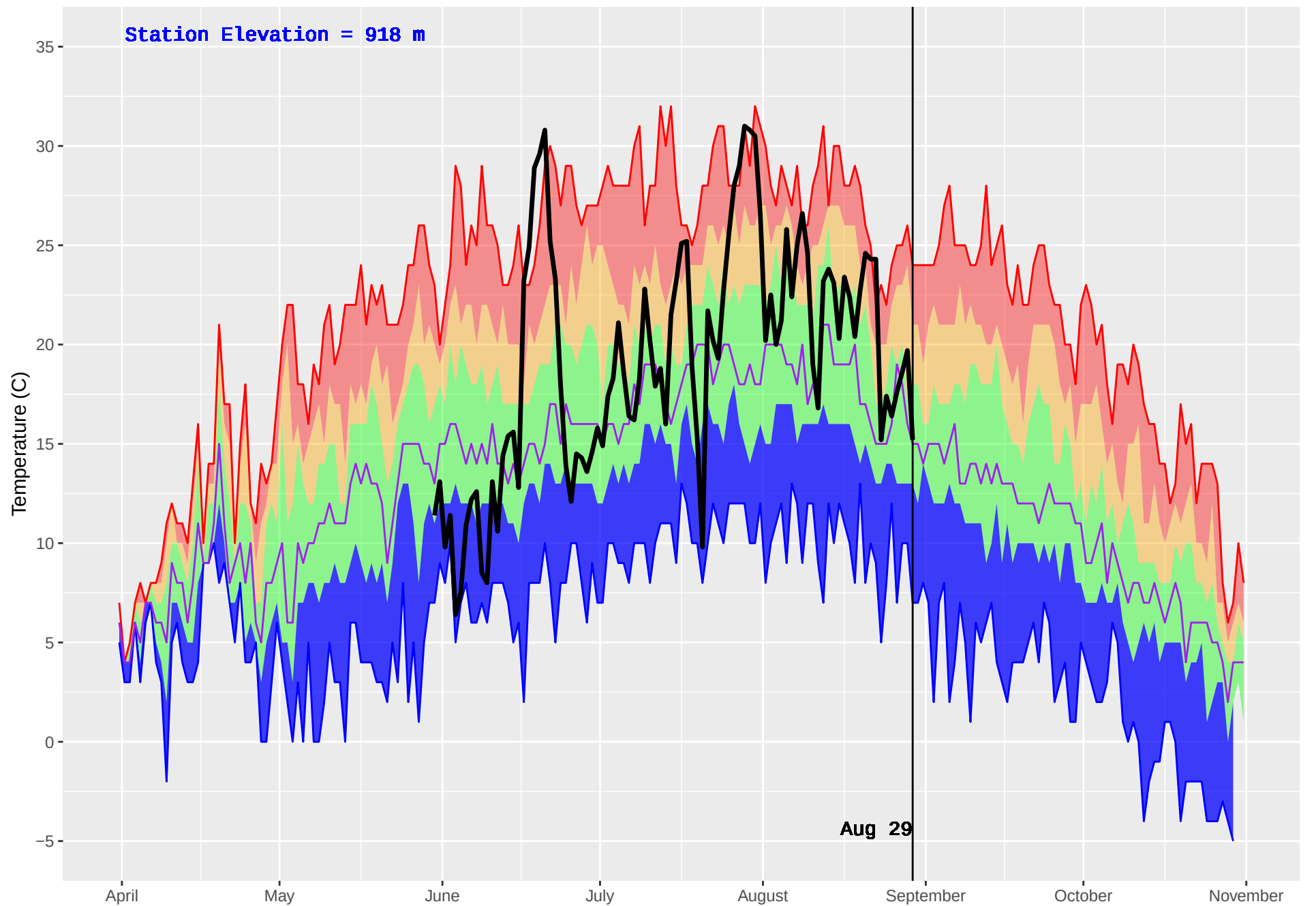
AUGIER LAKE (167) : Historical (1984–2016) and Current (2018) Daily Temperature
