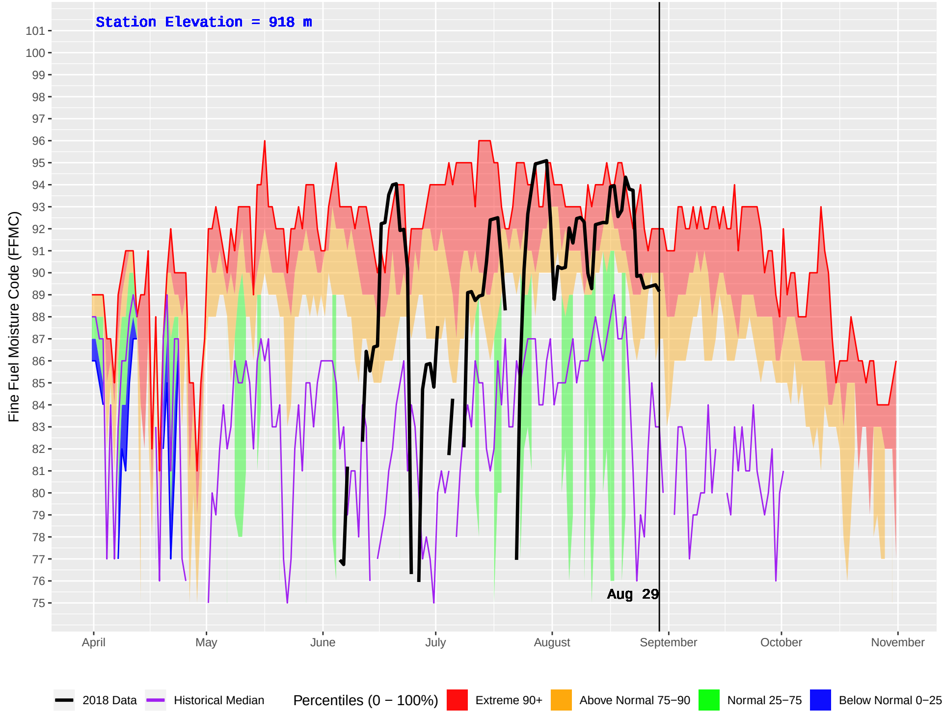
AUGIER LAKE (167) : Historical (1984–2016) and Current (2018) Daily Fine Fuel Moisture Code (FFMC)
